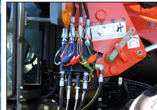
Auxiliary Valve Kit: Joystick control positioned to suit operator requirements.
