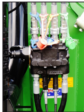
Auxiliary Valve Kit: Multi-position joystick control to suit individual operator requirements and compatible with a swivel seat.
