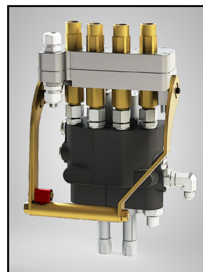
Auxiliary Valve Kit: Electric joystick control positioned to suit operator requirements. Loader connection is easy with a multi-coupler.
