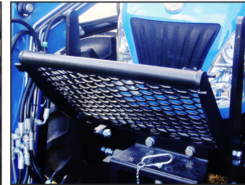
Guard Options: Protect the front of your investment with a grille guard or bump guard. The fold down grille guard insert creates a more compact and functional design.
